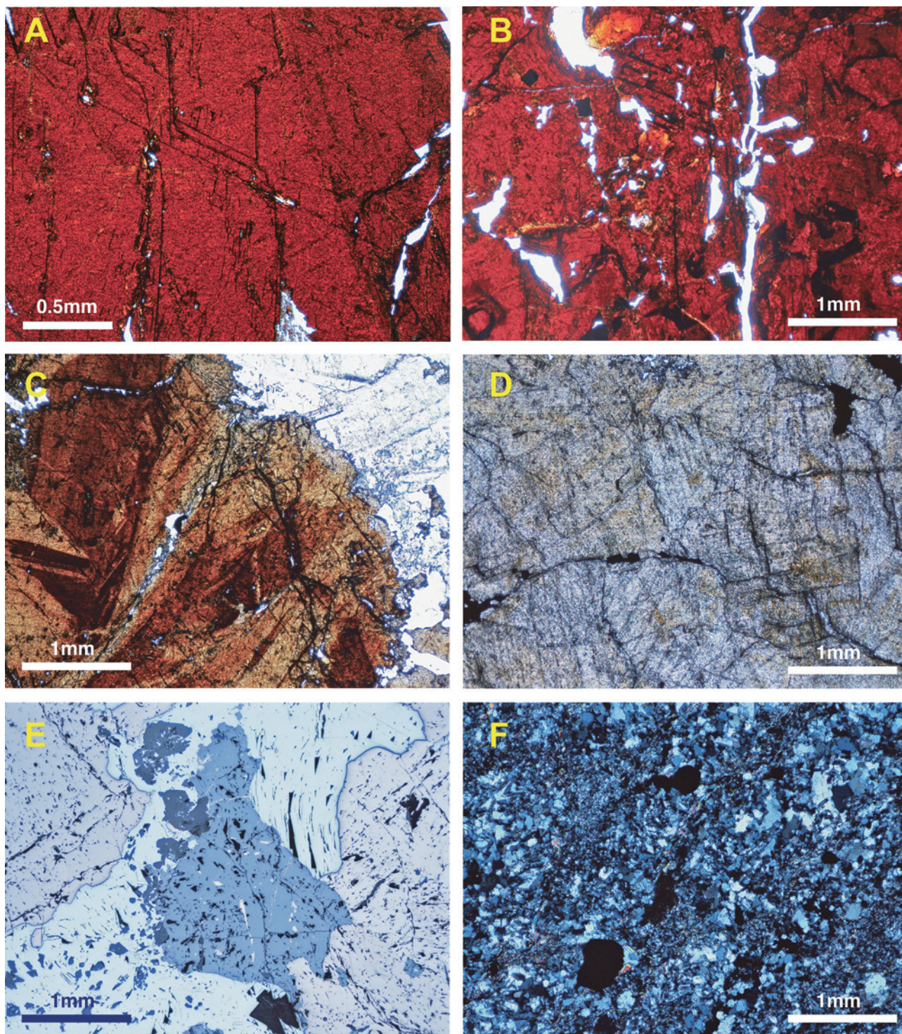
Plate II Microscopic pictures of selected minerals and rocks.
